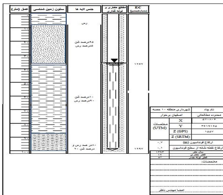
Figure 5. An example of drilling logs from the Isfahan-Borkhar study area (Isfahan Regional Water Company)
